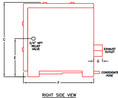
MUNCHKIN BOILER DIMENSIONS AND SPECIFICATIONS
