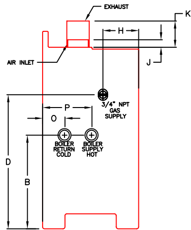
LEFT VIEW
