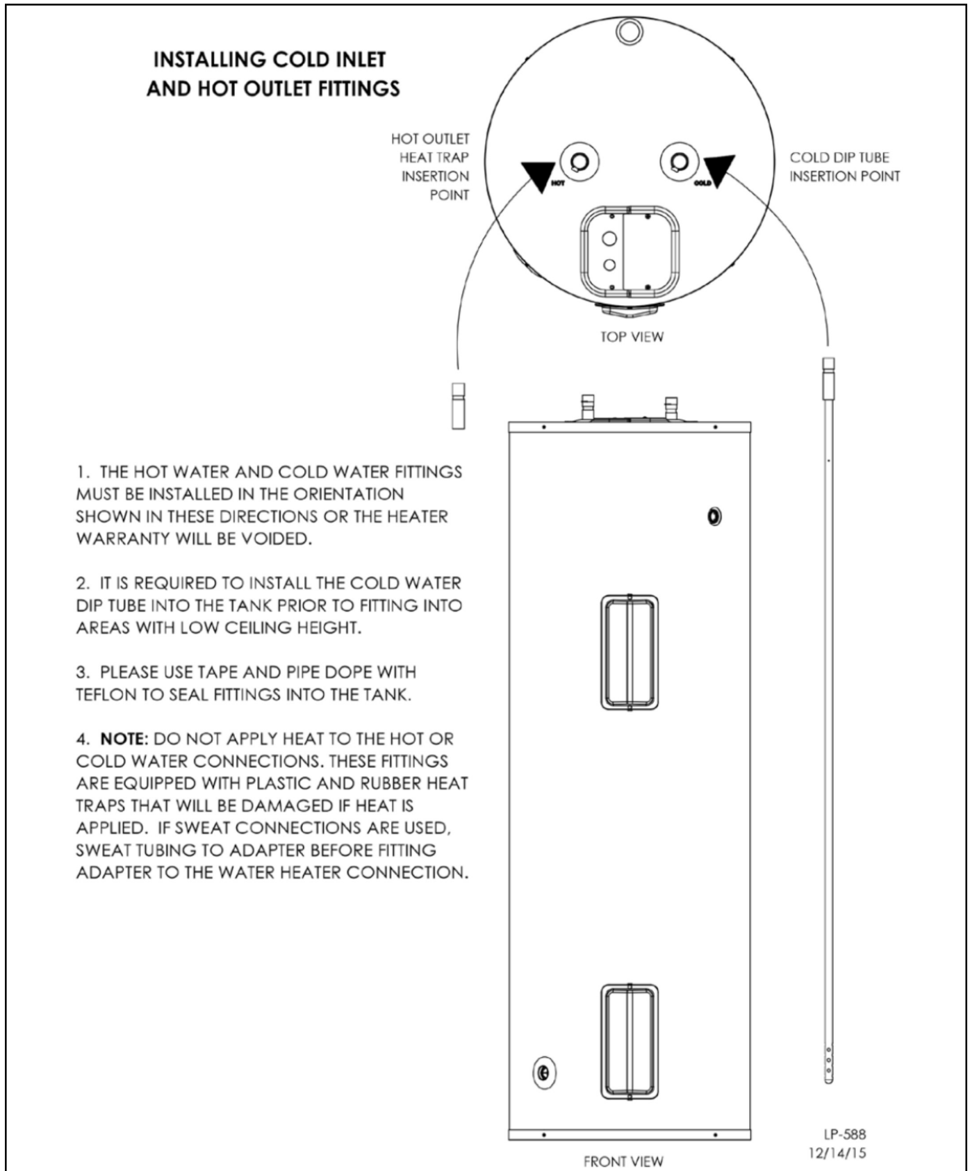
Figure 4 - Installing Cold Inlet and Hot Outlet Fittings
