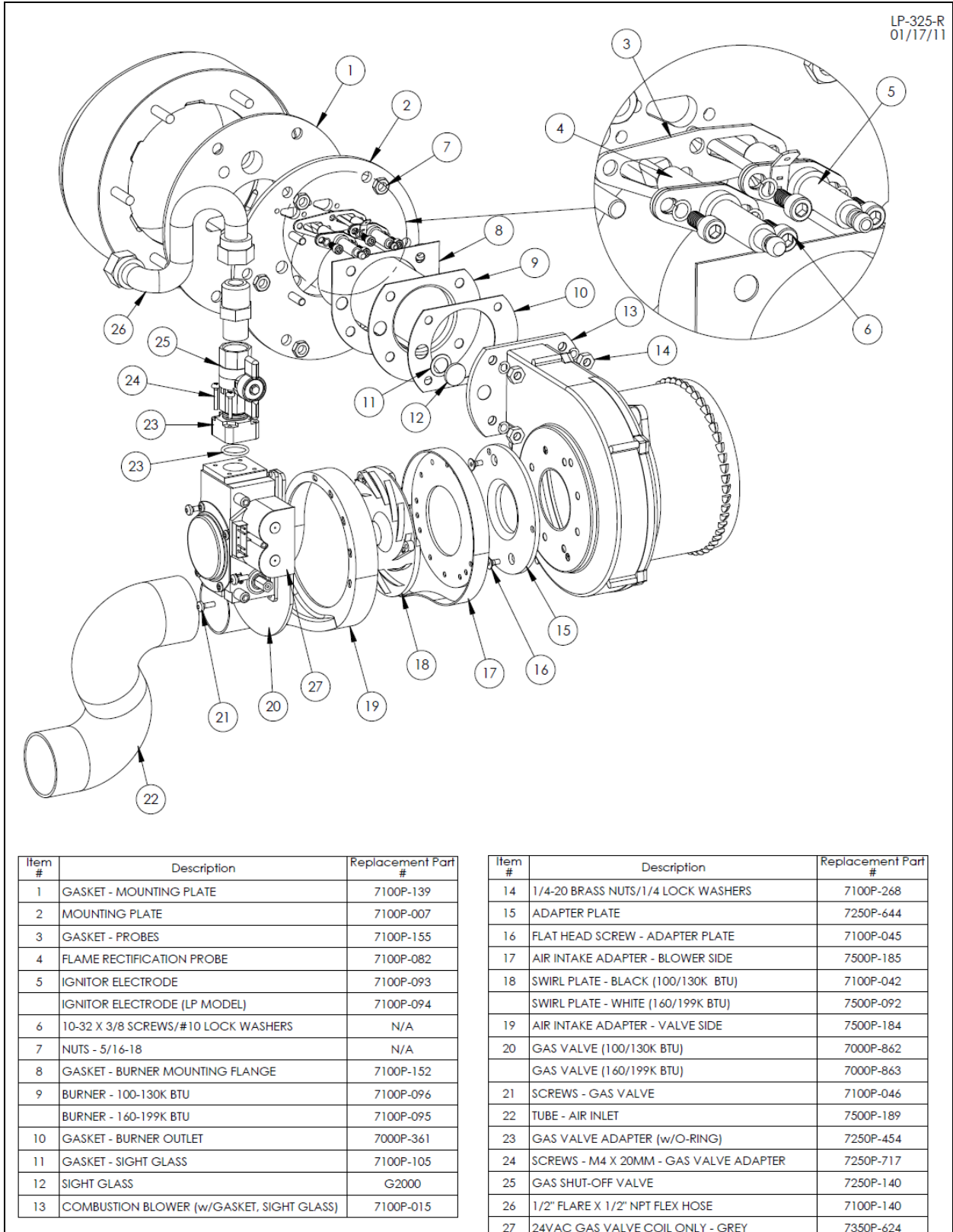
Figure 28 – Pioneer and Versa-Flame
