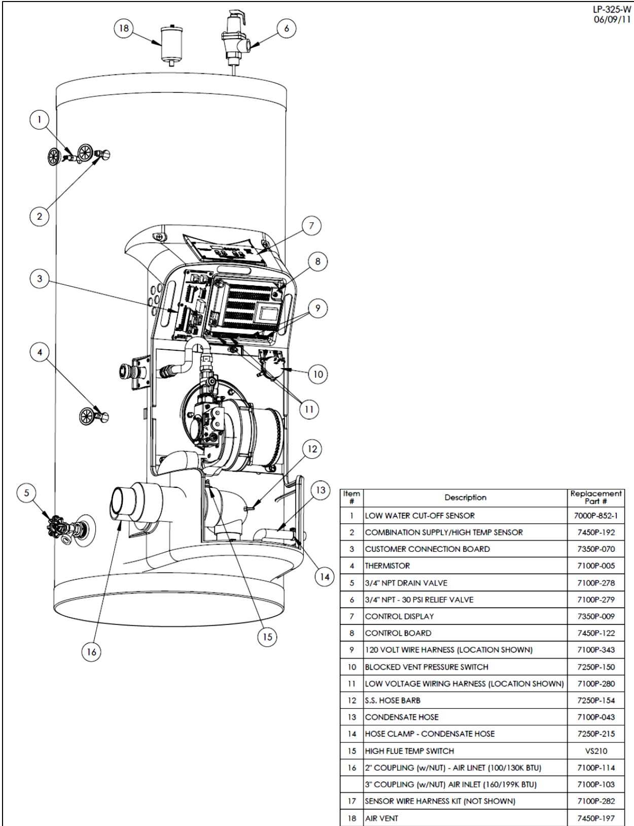
Figure 27 – Pioneer and Versa-Flame
