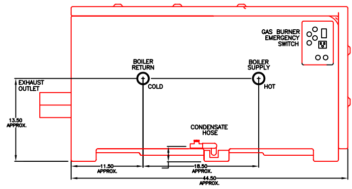
399 VWH LEFT SIDE VIEW
