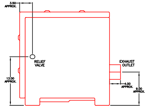
199 VWH RIGHT SIDE VIEW
