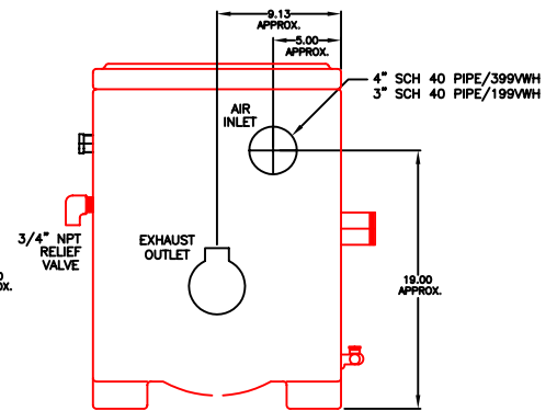
199 VWH/399 VWH BACK VIEW
