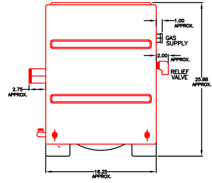
199VWH / 399 VWH FRONT VIEW
