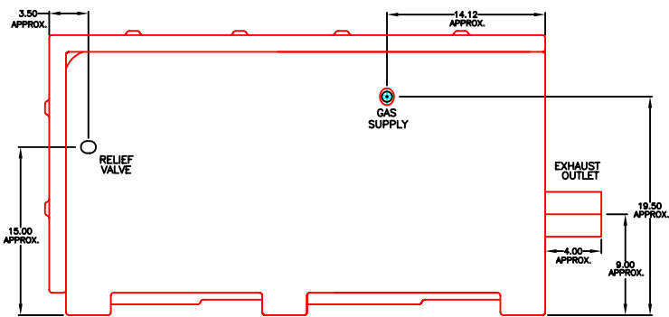
399 VWH RIGHT SIDE VIEW
