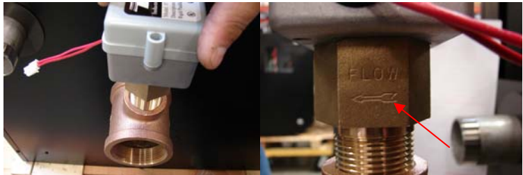
3. Thread switch into Tee using pipe dope, making certain the Flow Arrow points in the correct direction.
