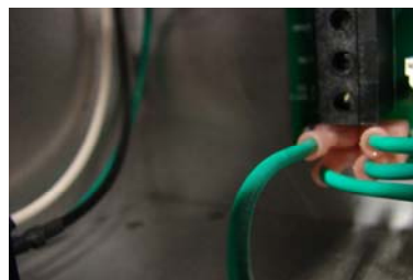
7. Once into the control box, Attach the Green ground to the Ground bus connection available.
