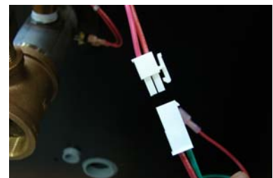
8. Connect wire harness To the Red Wire connection on The flow switch.
