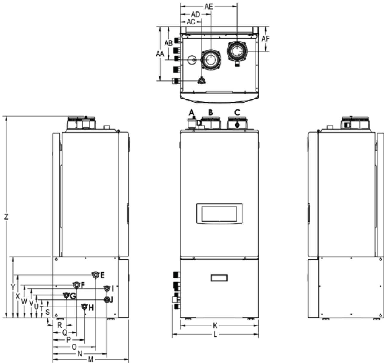
Figure 2 – Floor Mount Model Specifications and Dimensions
